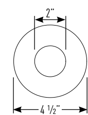
MXTG2-RFRR308 (1/2" Flat Mount with Lens)
